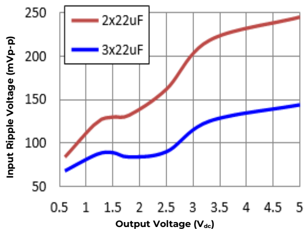
Figure 37. Input ripple voltage for various output voltages with 2x22 \mu\text{F} or 3x22 \mu\text{F} ceramic capacitors at the input (12A load). Input voltage is 12V.
