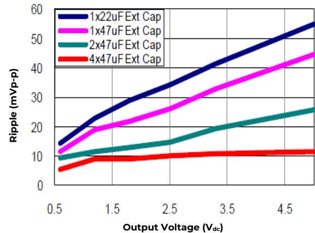
Figure 38. Output ripple voltage for various output voltages with external 1x22 \mu\text{F} , 1x47 \mu\text{F} , 2x47 \mu\text{F} or 4x47 \mu\text{F} ceramic capacitors at the output (12A load). Input voltage is 12V.
