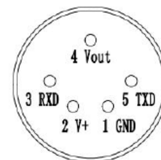
Fig3. Pin definition
