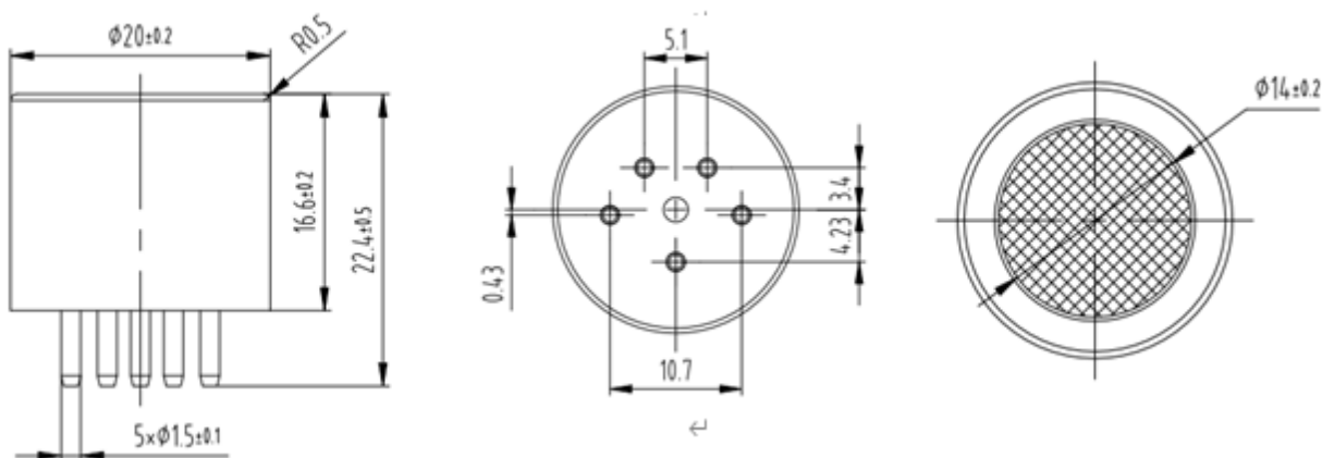
Fig2. Sensor structure (unmarked tolerance is ±0.2)
